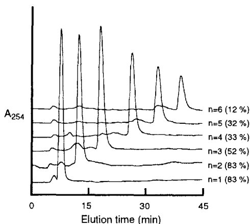
Figure 1. HPLC profile of the oligomanno-peptoids 2 (n=1-6). Erma ERC-NH-117 propylamino column; elution, CH 3 CN/H 2 O 4 to 1.5 with a gradient of 0.33 %/min.
