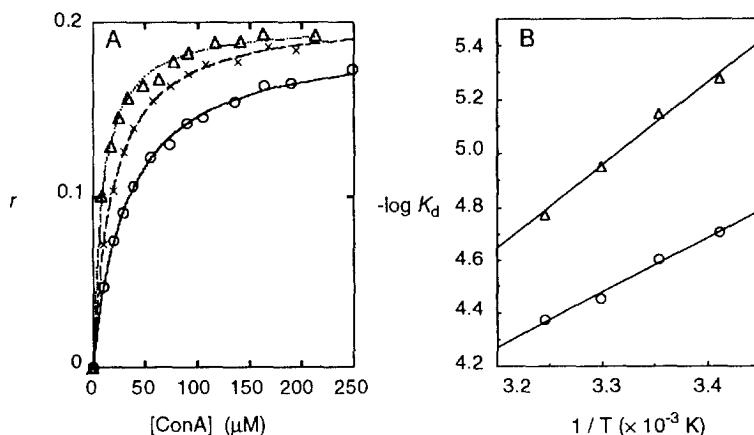
Figure 2. A) Titration curves of the fluorescence anisotropy assay for the binding of the oligomannopeptoids 2 ( n=1 ; O), ( n=2 ; x), ( n=3 ; Δ) to ConA and B) van't Hoff plots for the compounds 2 ( n=1 ; O), ( n=3 ; Δ).
